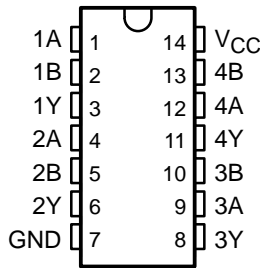
CD54AC08 ... F PACKAGE CD74AC08 ... E OR M PACKAGE (TOP VIEW)
