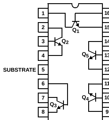
CA3183, CA3183A (PDIP, SOIC) TOP VIEW
