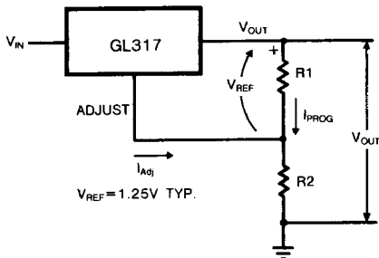
Fig. 1. Basic Circuit Configuration
