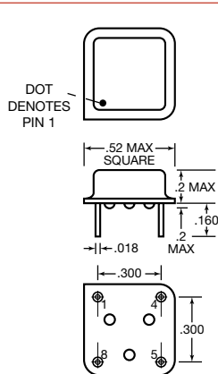
“H” Package
