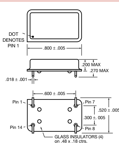
“M” Package with Gull Wing
