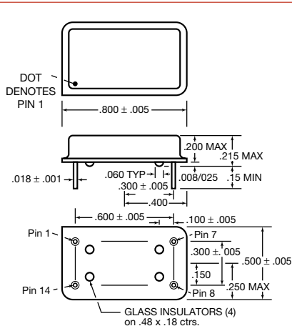
“M” Package – “L” Package is same as “M” but seated height is 0.190
