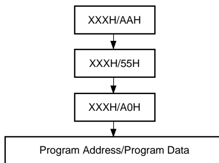
Figure 16 Embedded Program™ Algorithm
