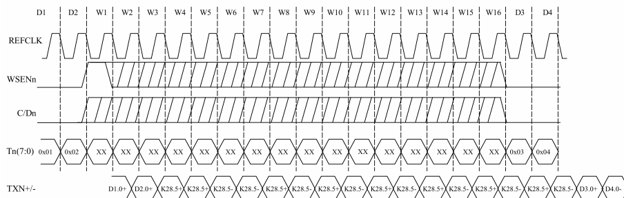
FIGURE 5. Word Sync Sequence Generation
