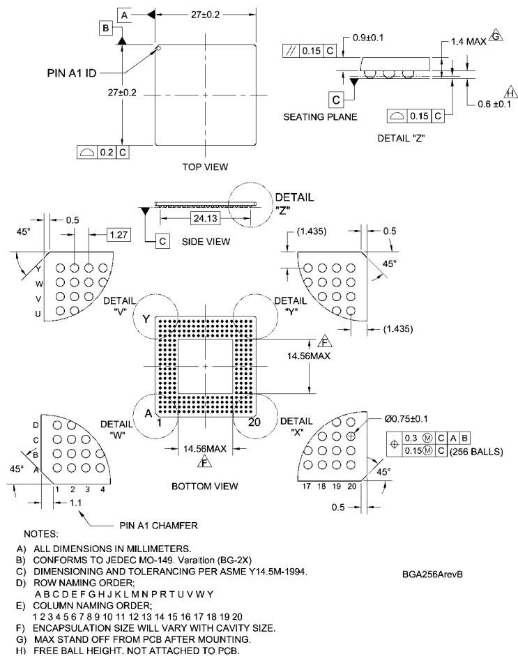
256-Ball Thermally-Enhanced Ball Grid Array (TBGA), JEDEC MO-149, 1.27mm Pitch, 27mm Square Package Number BGA256A
