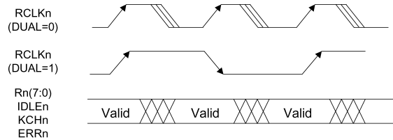
FIGURE 2. Transmit Timing, TMODE(2:0) = 000
