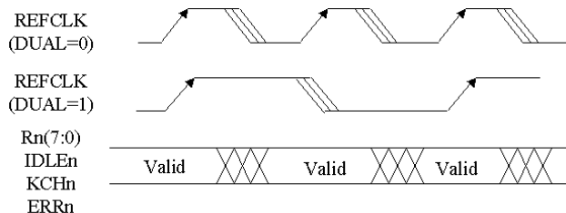
FIGURE 6. Receive Timing, RMODE(1:0) = 00 (REFCLK Centered)
