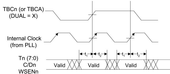
FIGURE 15. Transmit Input Timing Waveforms with TMODE = 10X
