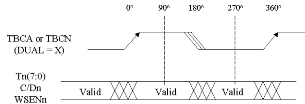
FIGURE 4. Transmit Timing, TMODE(2:0) = 11X
