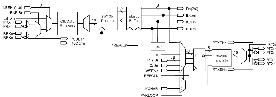
FIGURE 12. Parallel Loopback Mode Operation
