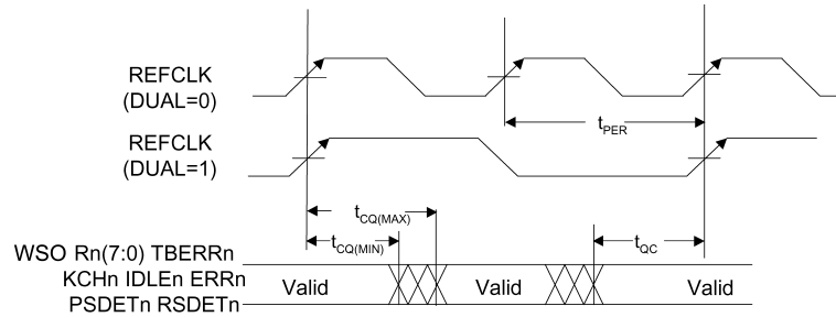
FIGURE 18. Receive Output Timing Waveforms with RMODE = 00 or 01
