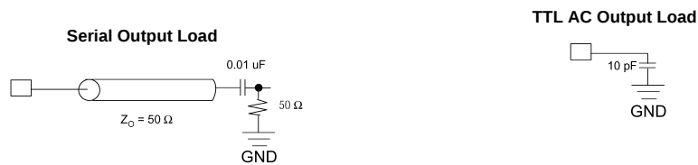
FIGURE 23. Parametric Test Load Circuit
