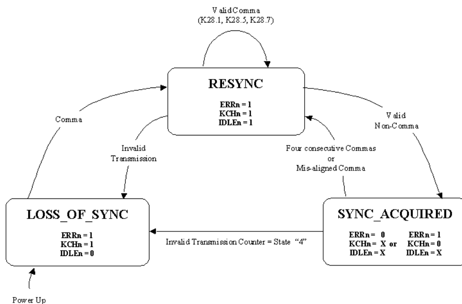
FIGURE 10. State Diagram of the Loss of Synchronization State Machine (see application note for more detail)
