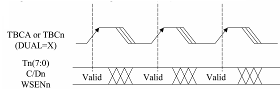
FIGURE 3. Transmit Timing, TMODE(2:0) = 10X
