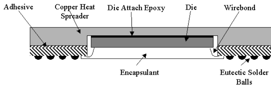
FIGURE 24. Thermal Resistance
