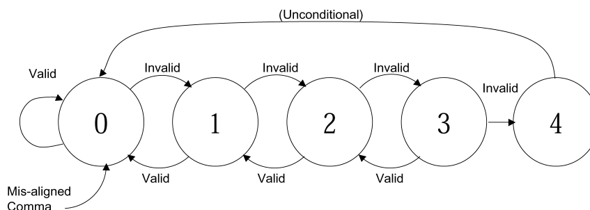
FIGURE 11. State Diagram of the Invalid Transmission counter
