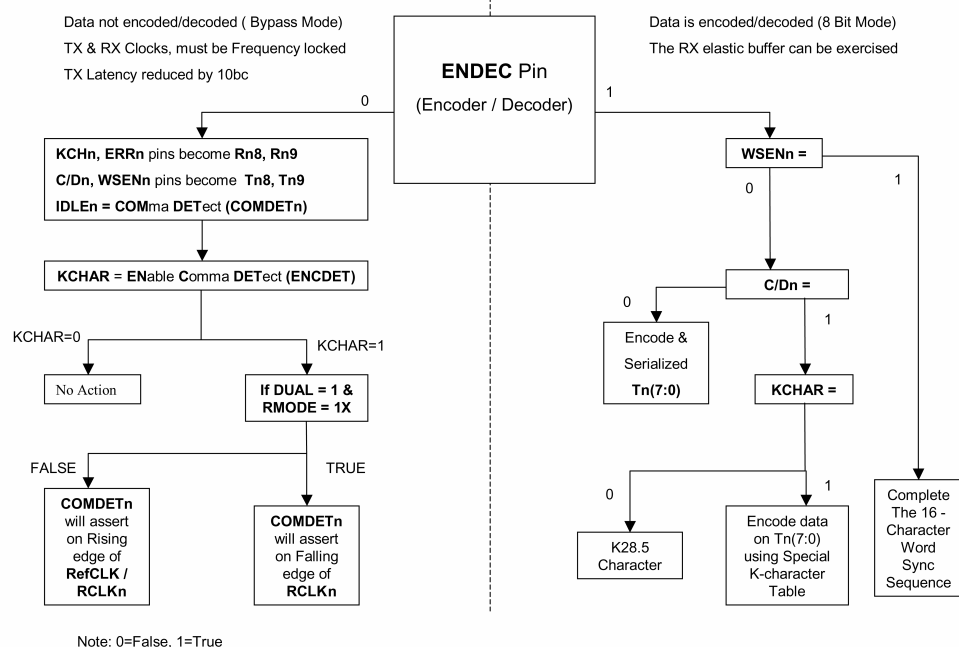
FIGURE 9. FIN7216-01 ENDEC Flow Control
