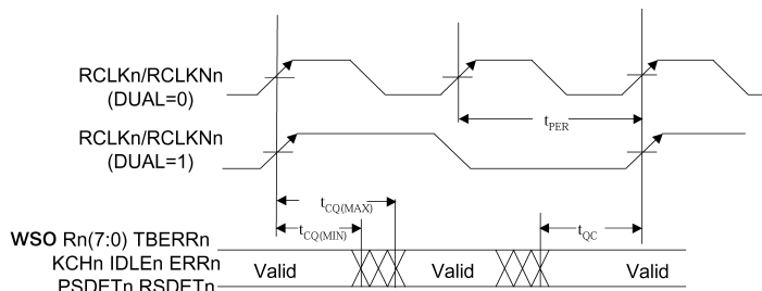
FIGURE 19. Receive Output Timing Waveforms with RMODE = 10 or 11
