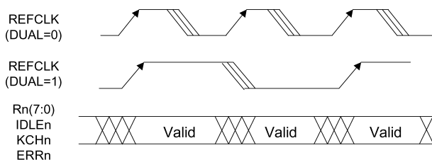
FIGURE 7. Receive Timing, RMODE(1:0) = 01 (REFCLK Leading)
