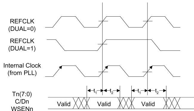
FIGURE 14. Transmit Input Timing Waveforms with TMODE = 000
