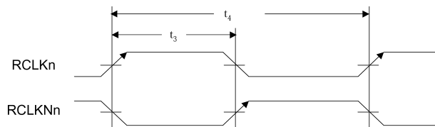
FIGURE 20. RCLKn and RCLKNn Timing Waveforms with DUAL = 1
