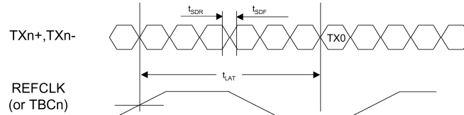
FIGURE 17. Transmit Serial Timing Waveforms
