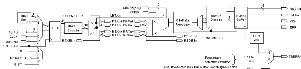
FIGURE 13. BIST Mode Operation
