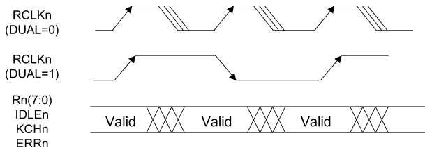
FIGURE 8. Receive Timing, RMODE(1:0) = 1X
