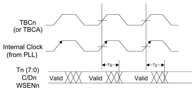
FIGURE 16. Transmit Input Timing Waveforms with TMODE = 11X (ASIC-Friendly Timing)
