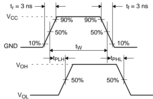
Figure 6. AC Waveforms
