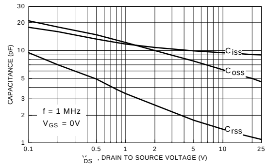
Figure 8. Capacitance Characteristics.
