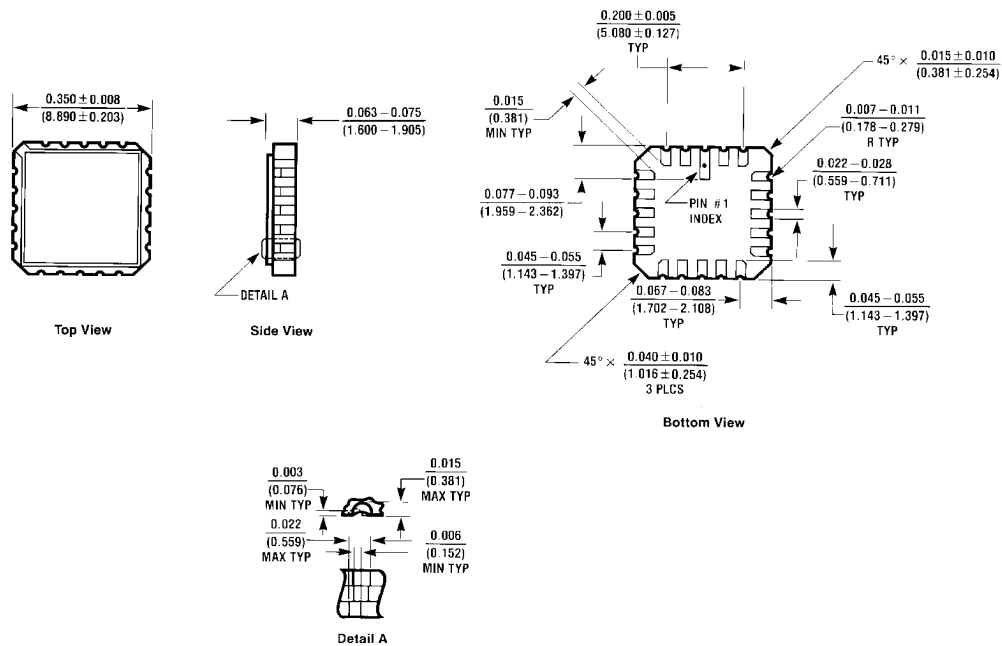
Ceramic Leadless Chip Carrier (E) Order Number 54LS174LMQB or 54LS175LMQB Package Number E20A
