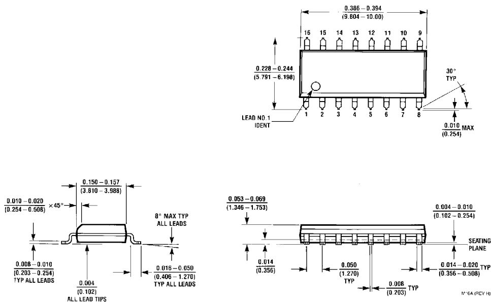
16-Lead Small Outline Molded Package (M) Order Number DM74LS174M or DM74LS175M Package Number M16A
