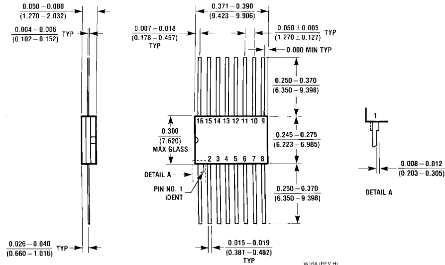
16-Lead Ceramic Flat Package (W) Order Number 54LS174FMB, 54LS175FMB, DM54LS174W or DM54LS175W Package Number W16A
