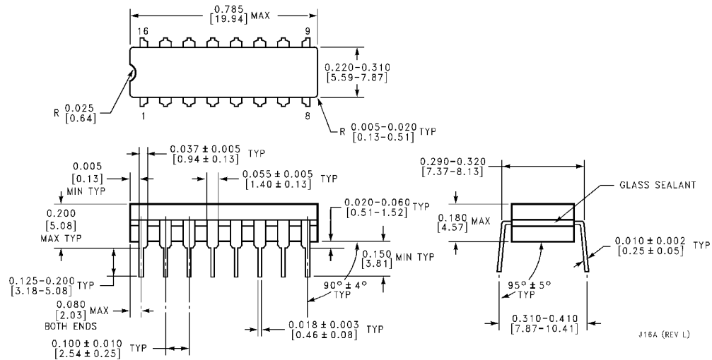
16-Lead Ceramic Dual-In-Line Package (J) Order Number DM54LS174DMQB, 54LS175DMQB, DM54LS174J or DM54LS175J Package Number J16A
