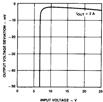
Line Regulation
