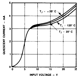
Quiescent Current
