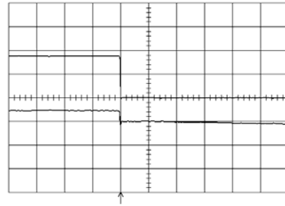
Shut-down enabled by disconnecting V_I at: T_{ref} = +25^\circ\text{C} , I_O = 10\text{ A} resistive load, V_I = 5.0\text{ V} . Top trace: output voltage (1.0 V/div.). Bottom trace: input voltage (2 V/div.). Time scale: 5.0 ms/div..
