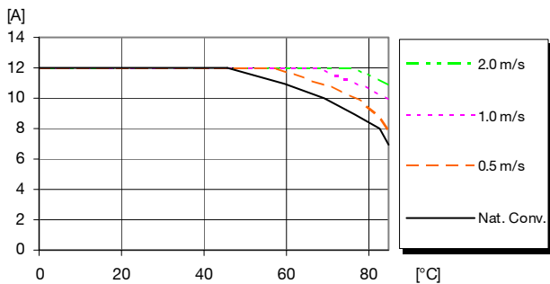
Available load current vs. ambient air temperature and airflow at V_I = 5.0 V, V_{OUT} = 3.3 V . See Thermal Consideration section.
