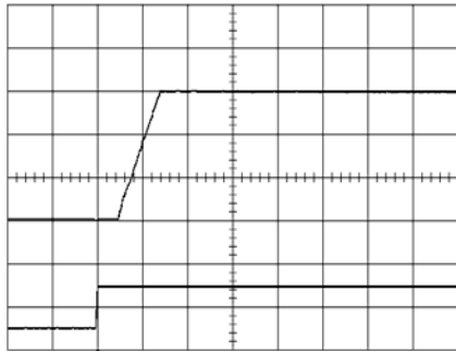
Start-up enabled by connecting V_i at: T_{ref} = +25^\circ\text{C} , I_O = 10\text{ A} resistive load, V_i = 5.0\text{ V} . Top trace: output voltage (0.5 V/div.). Bottom trace: input voltage (5 V/div.). Time scale: 5 ms/div..
