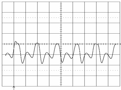
Output voltage ripple (20mV/div.) at: T_{ref} = +25^\circ\text{C} , I_O = 10\text{ A} resistive load, V_i = 5.0\text{ V} . Time scale: 2 μs/div. See the filter in the Output ripple and noise section (EMC Specification).
