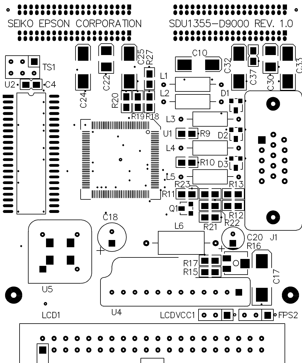
Figure 6-1: Component Placement
