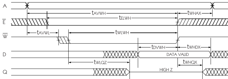
Write Cycle 1, \overline{W} Controlled
