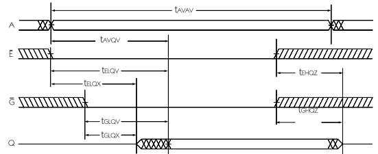
Read Cycle 2 ( \overline{W} High)
