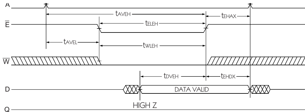
Write Cycle 2, \overline{E} Controlled
