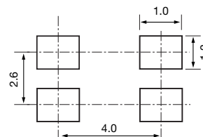
Figure 2) Land Pattern
