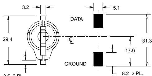
DS9094FS RECOMMENDED PAD SIZE
