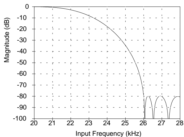
Figure 17. CS5336 Digital Filter Transition Band
