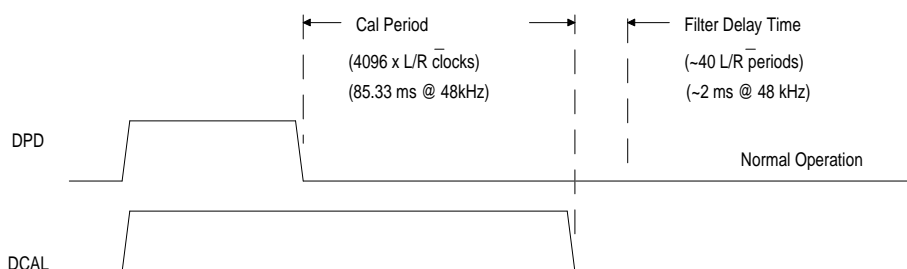
Figure 6. Initial Calibration Cycle Timing
