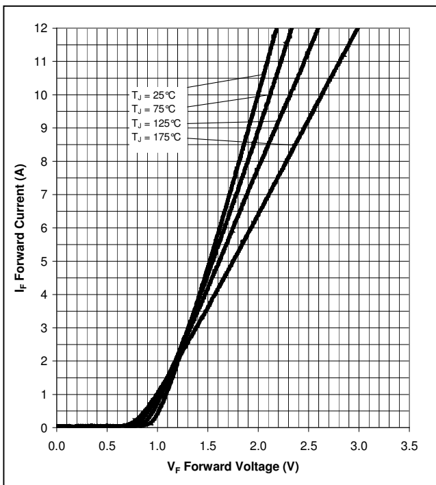
Figure 1. Forward Characteristics
