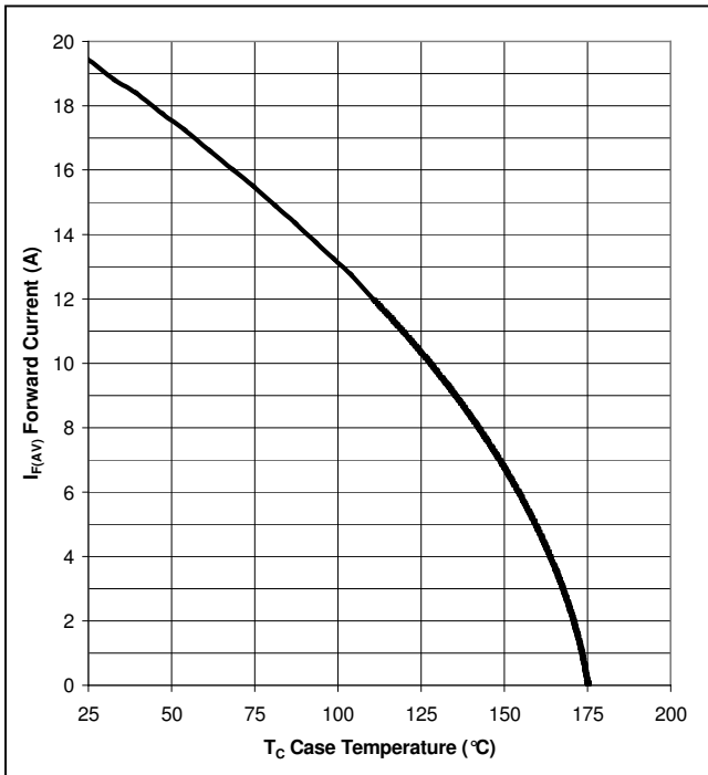
Figure 3. Current Derating
