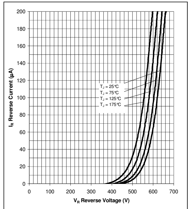
Figure 2. Reverse Characteristics
