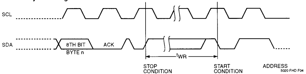
Figure 3. Start/Stop Timing
