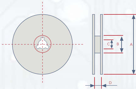
- 7" Reel Dimensions - 16mm Tape
