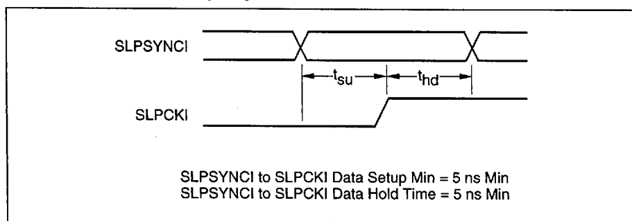
Figure 13. SLPSYNCI Timing Diagram
