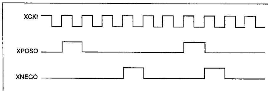
Figure 6. Transmitter Output
