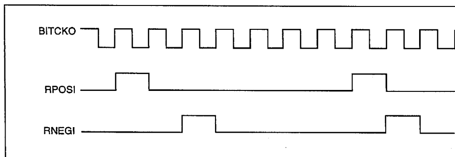
Figure 7. Clocked Receiver Input
