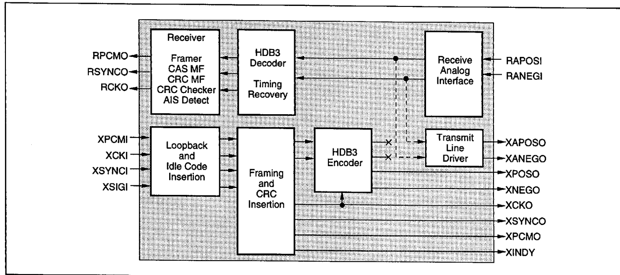
Figure 15. Line Loopback
