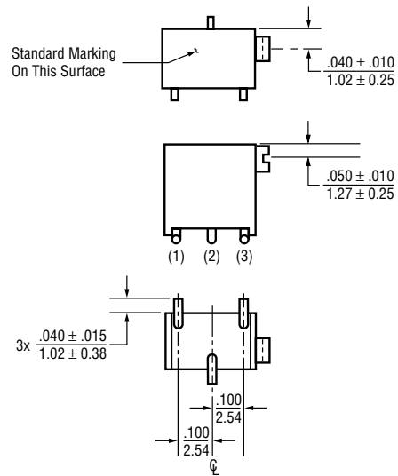
Recommended PCB Layout - Models 84W and 84X
