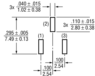
Recommended PCB Layout - Models 84W and 84X
