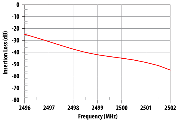
Figure 7. Attenuation, 2496 – 2502 MHz
