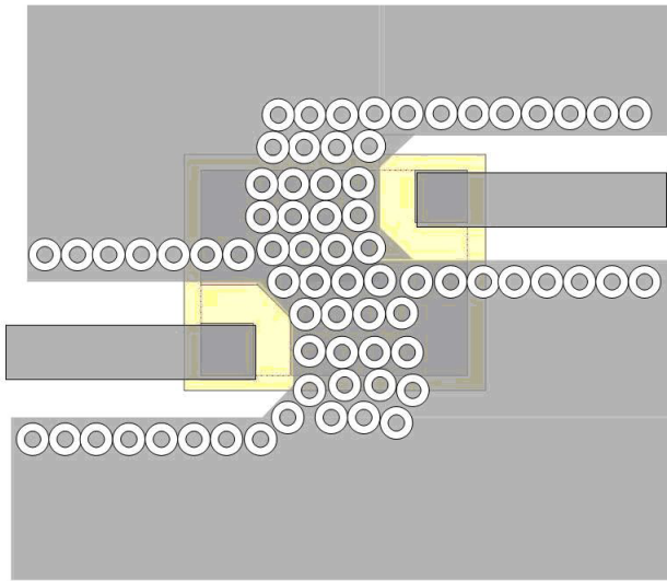
Figure 16. ACPF-7024 Superposed on PCB Layout (top view)
