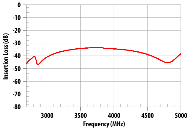
Figure 9. Attenuation, 2690 – 5000 MHz
