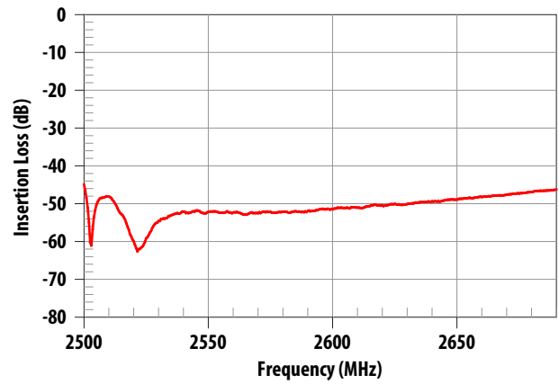
Figure 8. Rejection in 2.5 GHz WiMAX and LTE Band 7 (2500 – 2690 MHz)
