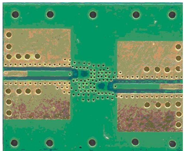
Figure 20. Evaluation board (SMA connectors) for ACPF-7024, bottom view
