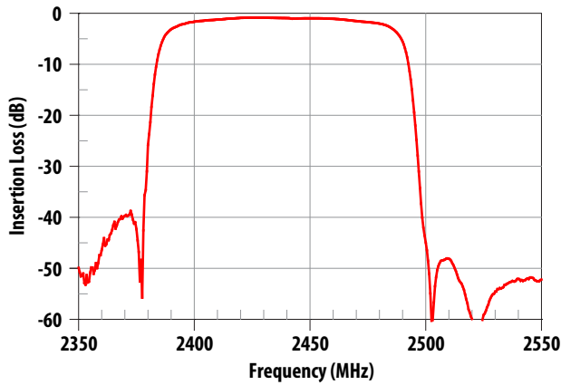
Figure 3. Attenuation, 2350 – 2550 MHz
