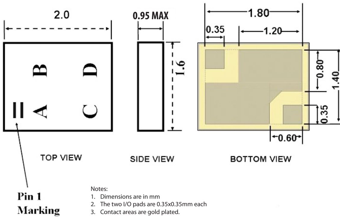
Figure 13. Package Outline Drawing
