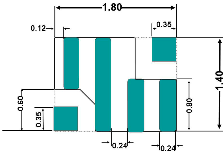
Figure 17. Recommended Solder Stencil (top view)
