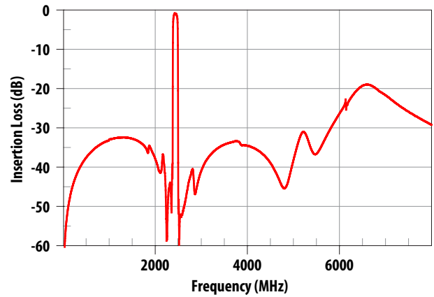
Figure 4. Wideband Attenuation, 0.05 – 8000 MHz
