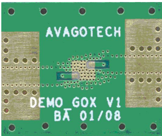
Figure 19. Evaluation board (SMA connectors) for ACPF-7024, top view
