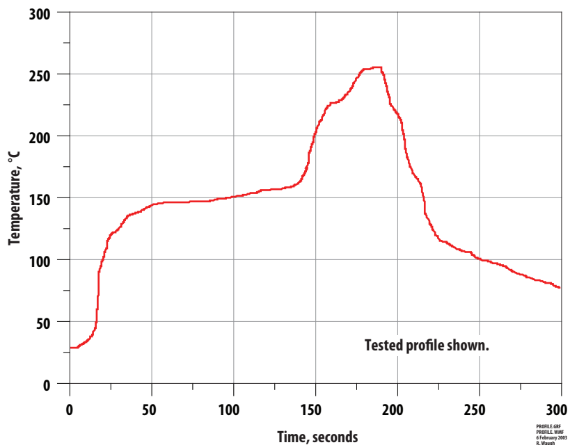
Figure 24. Verified SMT Solder Profile
