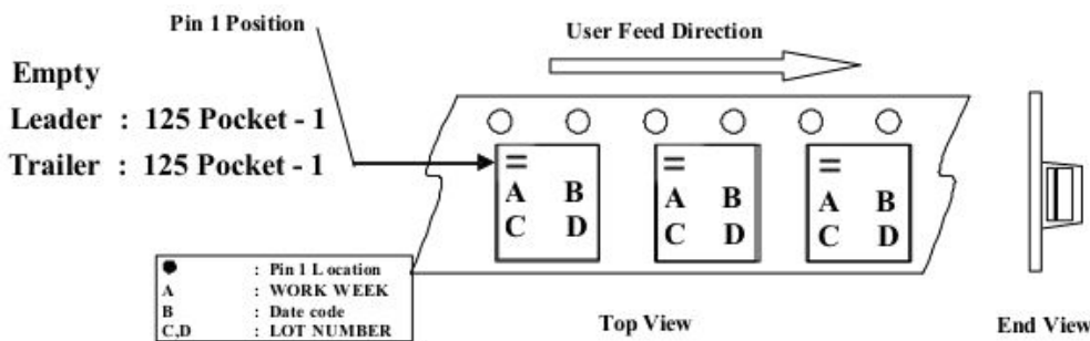
Figure 22. Orientation in Tape
