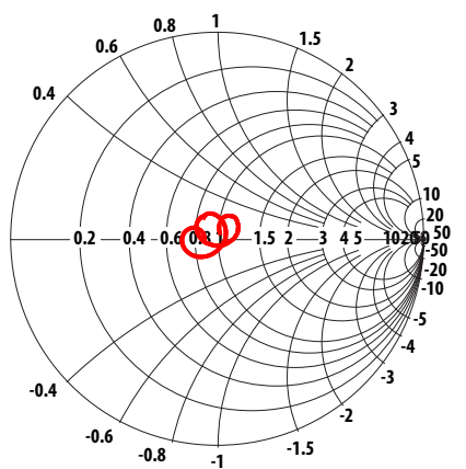
Figure 11. Input Port Impedance, 2400 – 2482 MHz
