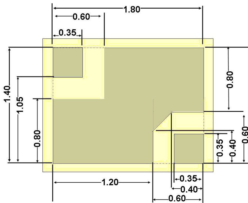
Figure 14. Bottom View Detail (mm)
