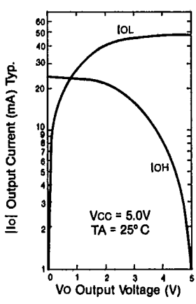
Figure 3. Output Drive Currents
