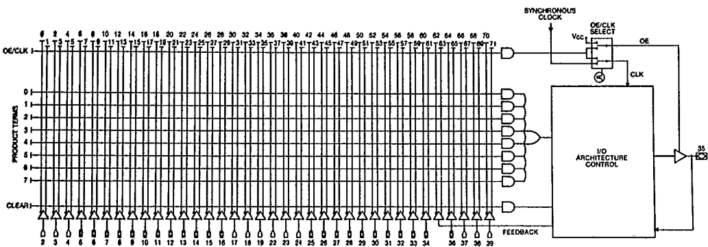
Figure 1. Logic Array Macrocell
