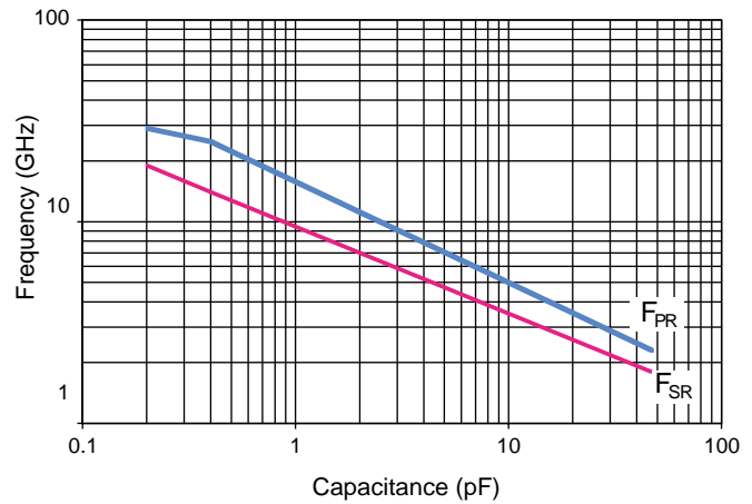
650S FSR & FPR
