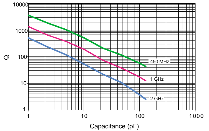
650F Q vs Capacitance
