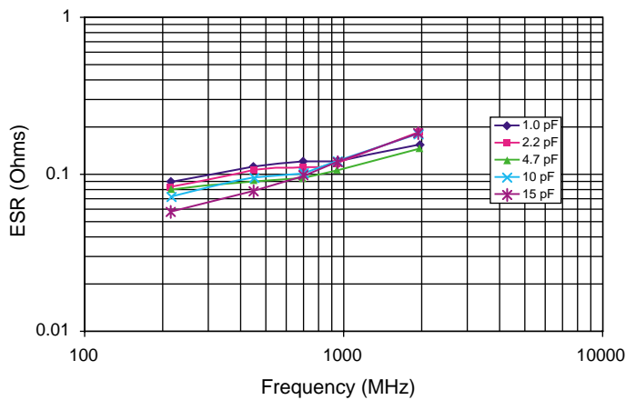
650L ESR vs Frequency
