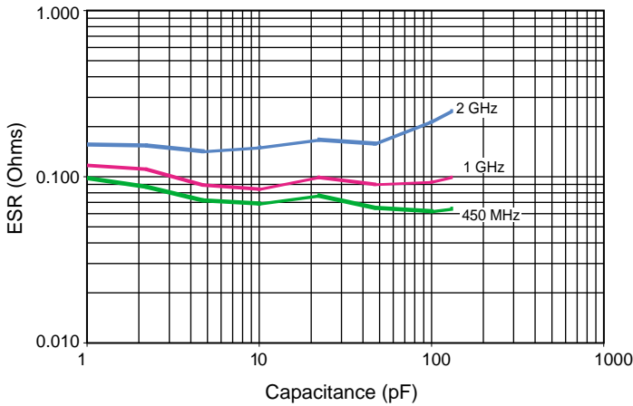
650F ESR vs Capacitance
