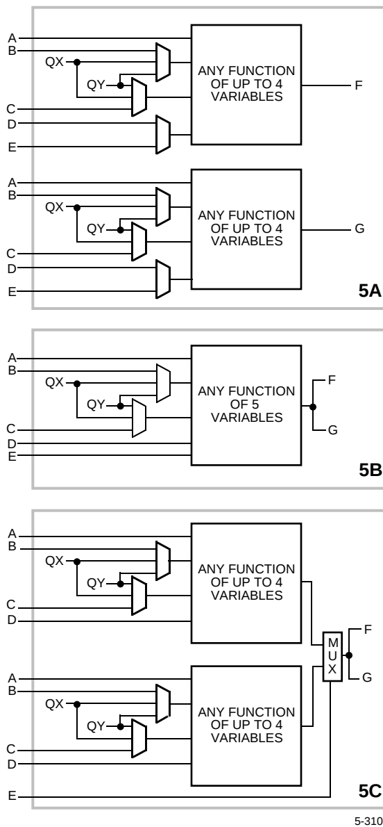
Configurable Logic Block (continued)
