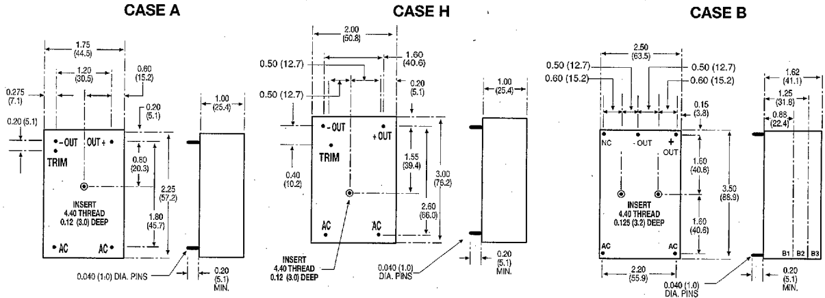
ALL DIMENSIONS IN INCHES (mm)
