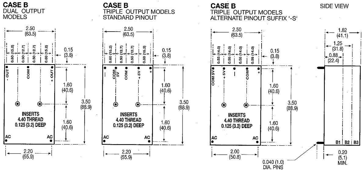
ALL DIMENSIONS IN INCHES (mm)
