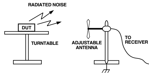
Figure 24. Radiated Emissions Test Setup
