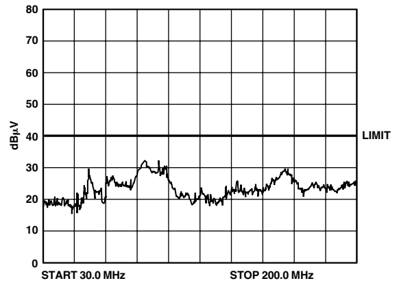
TPC 4. EMC Radiated Emissions
