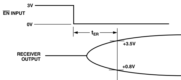
Figure 13. Receiver-Disable Timing
