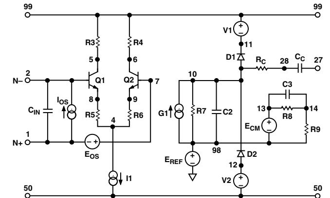
Figure 17. SPICE Macro-Model Input and Gain Stage
