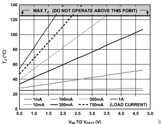
Figure 38. 0 mm² of PCB Copper, T_A = 25^\circ\text{C} , SOIC
