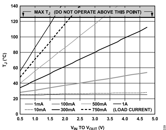
Figure 40. 100 mm² of PCB Copper, T_A = 25^\circ\text{C} , LFCSP
