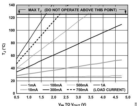
Figure 39. 500 mm² of PCB Copper, T_A = 25^\circ\text{C} , LFCSP
