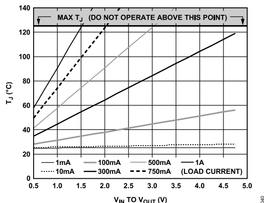
Figure 41. 0 mm² of PCB Copper, T_A = 25^\circ\text{C} , LFCSP
