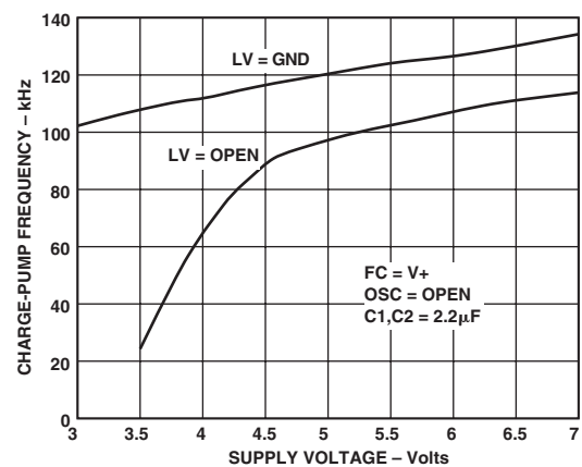
TPC 12. Charge-Pump Frequency vs. Supply Voltage
