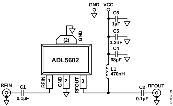
Figure 20. Evaluation Board Schematic
