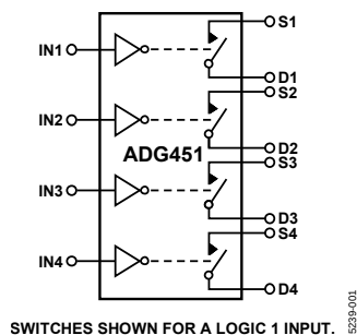
Figure 1. ADG451
