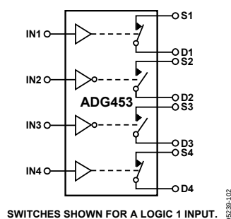
Figure 3. ADG453
