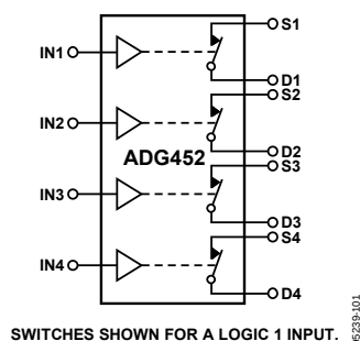
Figure 2. ADG452
