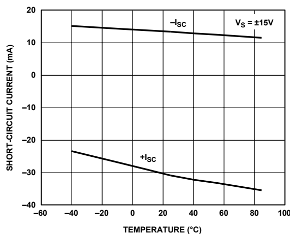
Figure 18. Short-Circuit Current vs. Temperature
