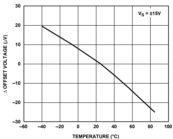
Figure 21. \Delta Offset Voltage vs. Temperature
