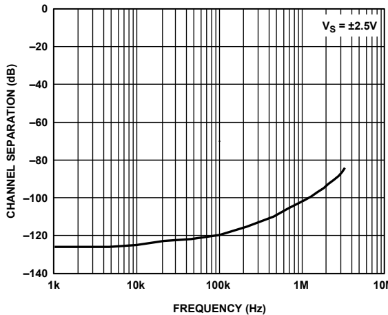
Figure 48. Channel Separation
