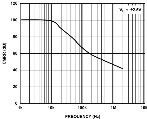
Figure 36. CMRR vs. Frequency
