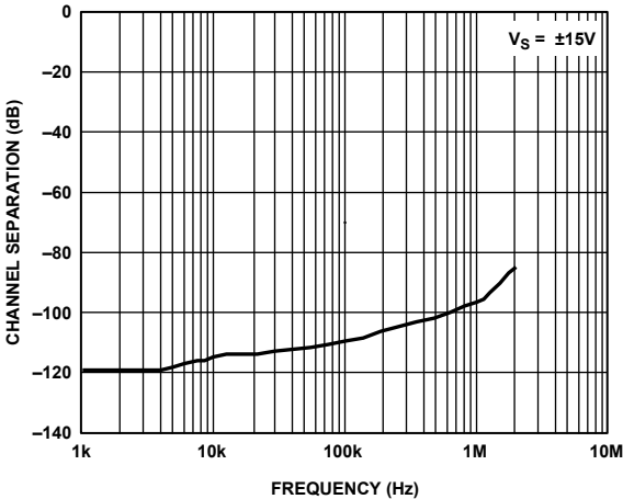
Figure 27. Channel Separation
