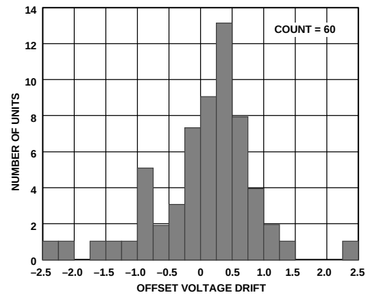
Figure 14. TC V_{OS} Distribution, -55^{\circ}\text{C} to +125^{\circ}\text{C} , V_S = 5, 0
