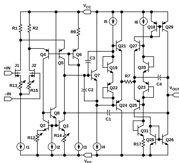
AD824 Die Size 0.70 X 0.130 inch, 9,100 sq. mils. Substrate (Die Backside) Is Connected to V_+ . Transistor Count, 143.
