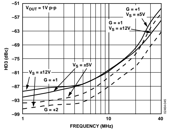
Figure 44. AD8130 Third Harmonic Distortion vs. Frequency
