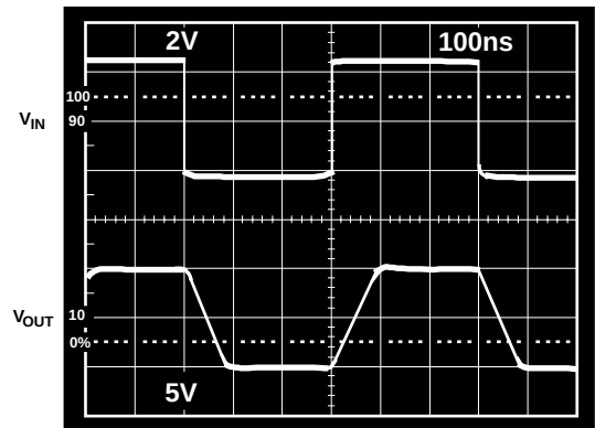
Figure 41. Output Waveform of an AD811 Driving a 500 pF Load. Gain = +2, R_{FB} = 649 \Omega , R_S = 15 \Omega , R_L = 10 \text{ k}\Omega
