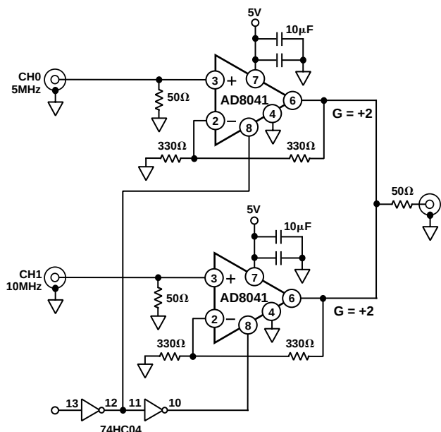
Figure 7. 2:1 Multiplexer
