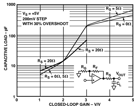
Figure 41. Capacitive Load Drive vs. Closed-Loop Gain
