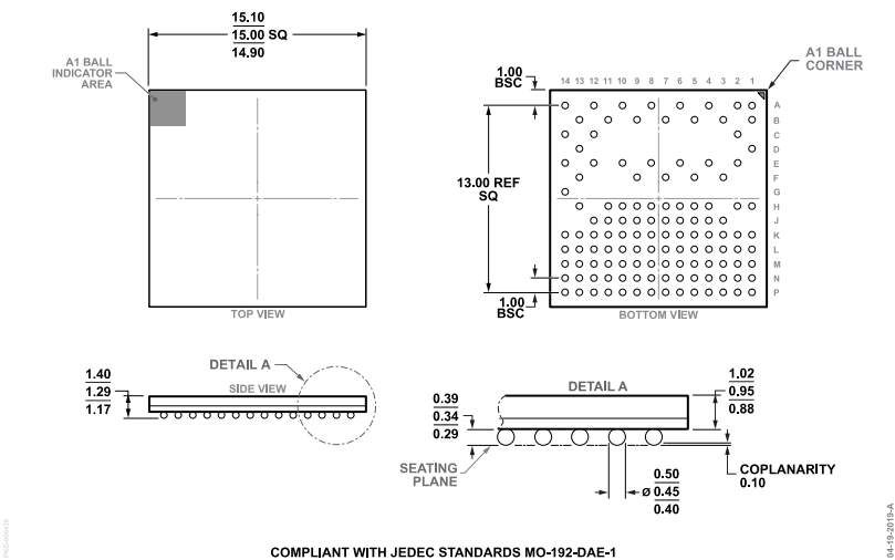
Figure 20. 124-Lead Chip Scale Package Ball Grid Array [CSP_BGA] (BC-124-4) Dimensions shown in millimeters
