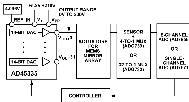
Figure 18. AD45335 in a MEMS-Based Optical Switch
