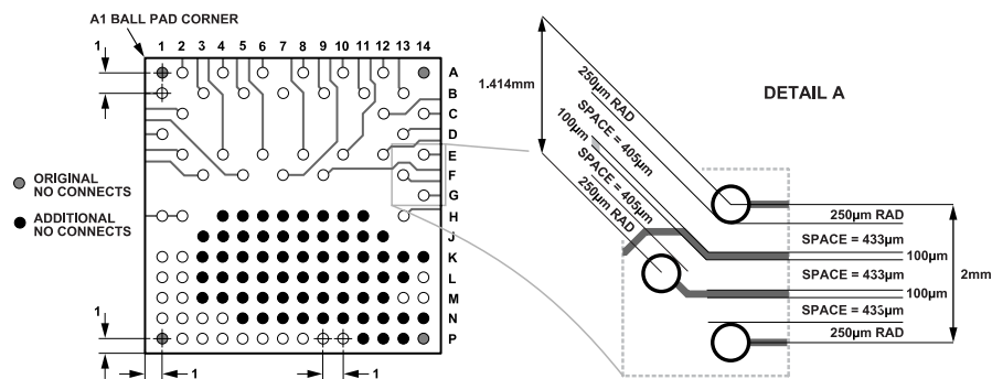
Figure 19. Layout Guidelines to Comply with IPC-221
