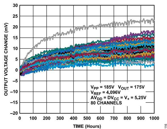
Figure 16. Long-Term Output Voltage Drift Over 1000 Hours at 80°C
