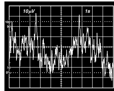
Figure 10. 0.1 Hz to 10 Hz Voltage Noise
