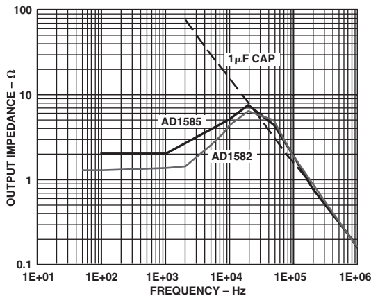
Figure 8b. Output Impedance vs. Frequency
