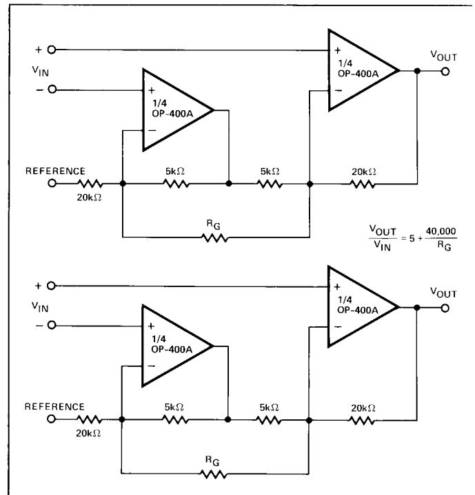
FIGURE 1: Dual Low-Power Instrumentation Amplifier
