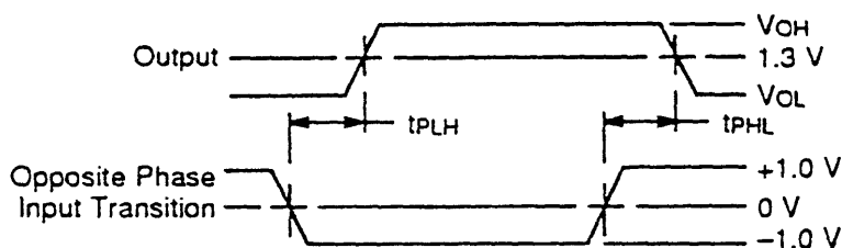
Propagation Delay (Notes 1 and 3)
