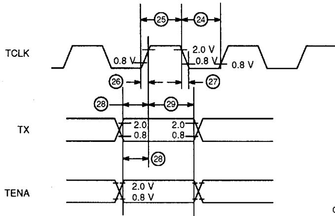
TCLK and TX Timing
