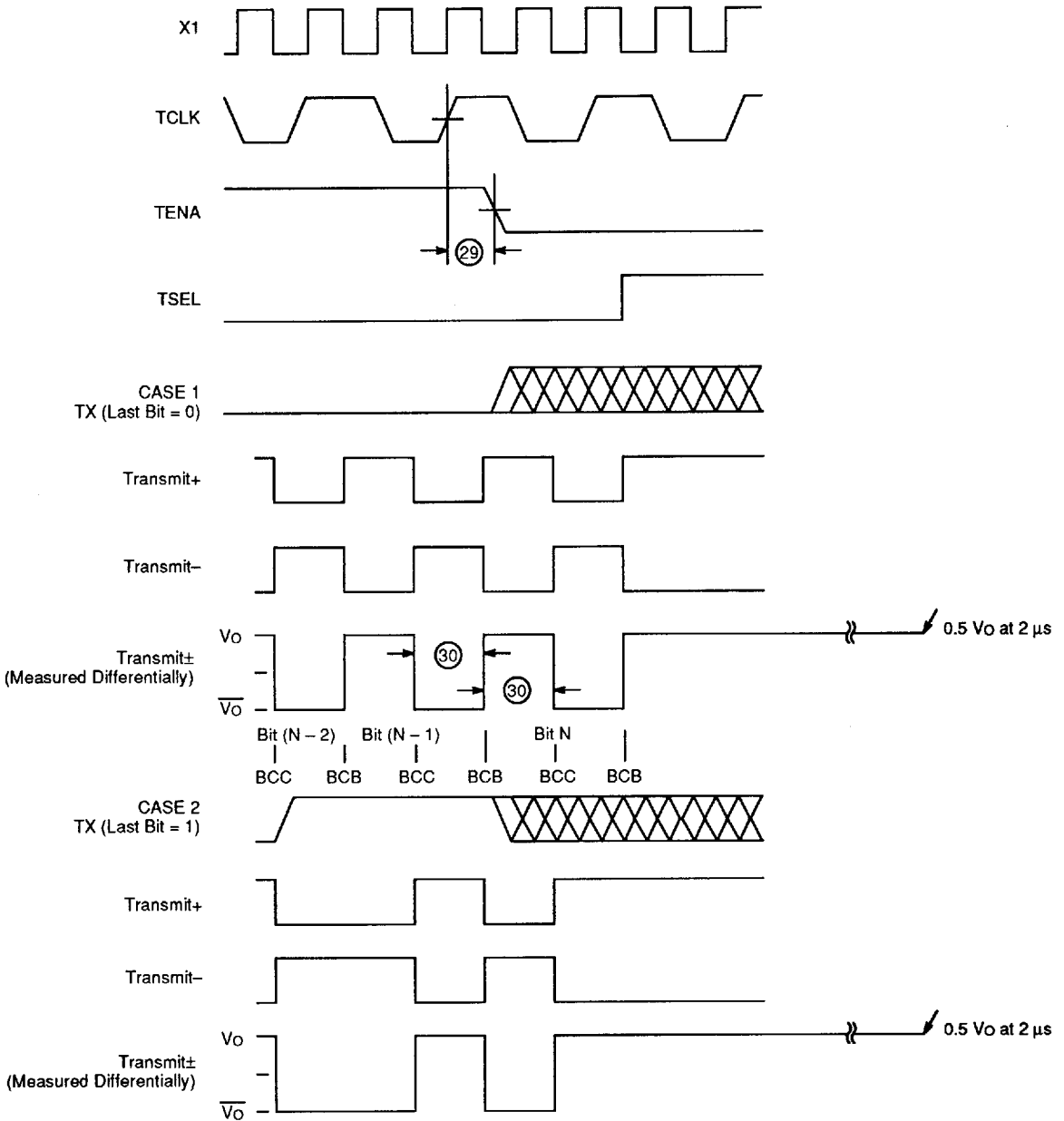
Transmit Timing – End of Transmission*
