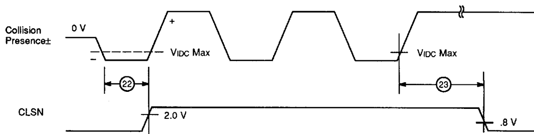
Collision Timing
