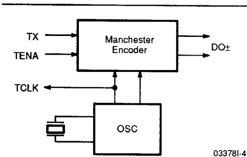
Figure 1. Transmit Section
