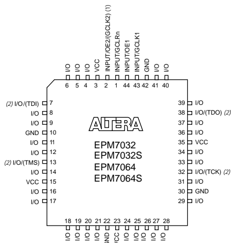
44-Pin PLCC
