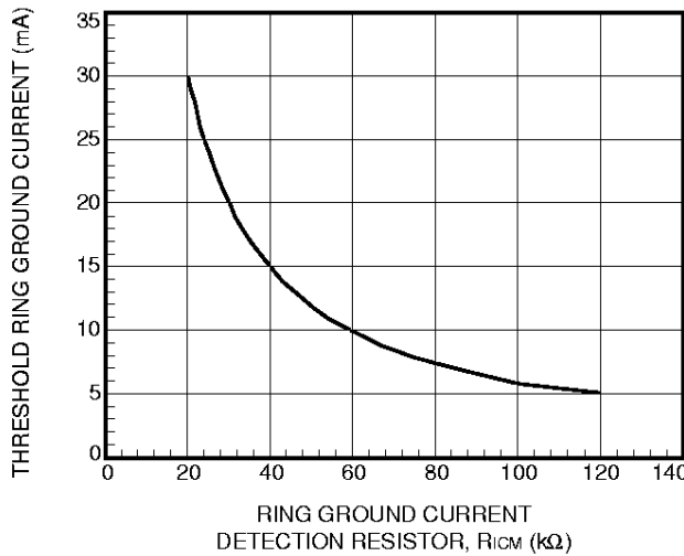
Figure 17. Ring Ground Detection Programming
