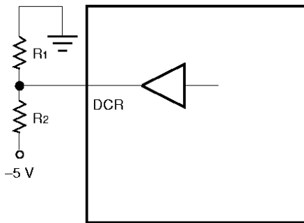
Figure 24. Equivalent Circuit for Adjusting the Overhead Voltage
