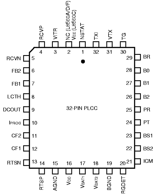
Figure 2. 32-Pin Diagram (PLCC Chip)
