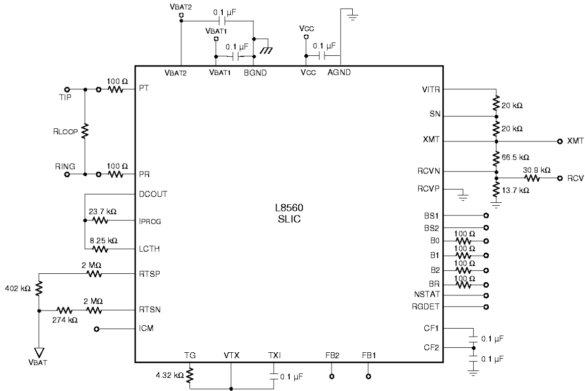
Figure 5. Basic Test Circuit (44-Pin PLCC)
