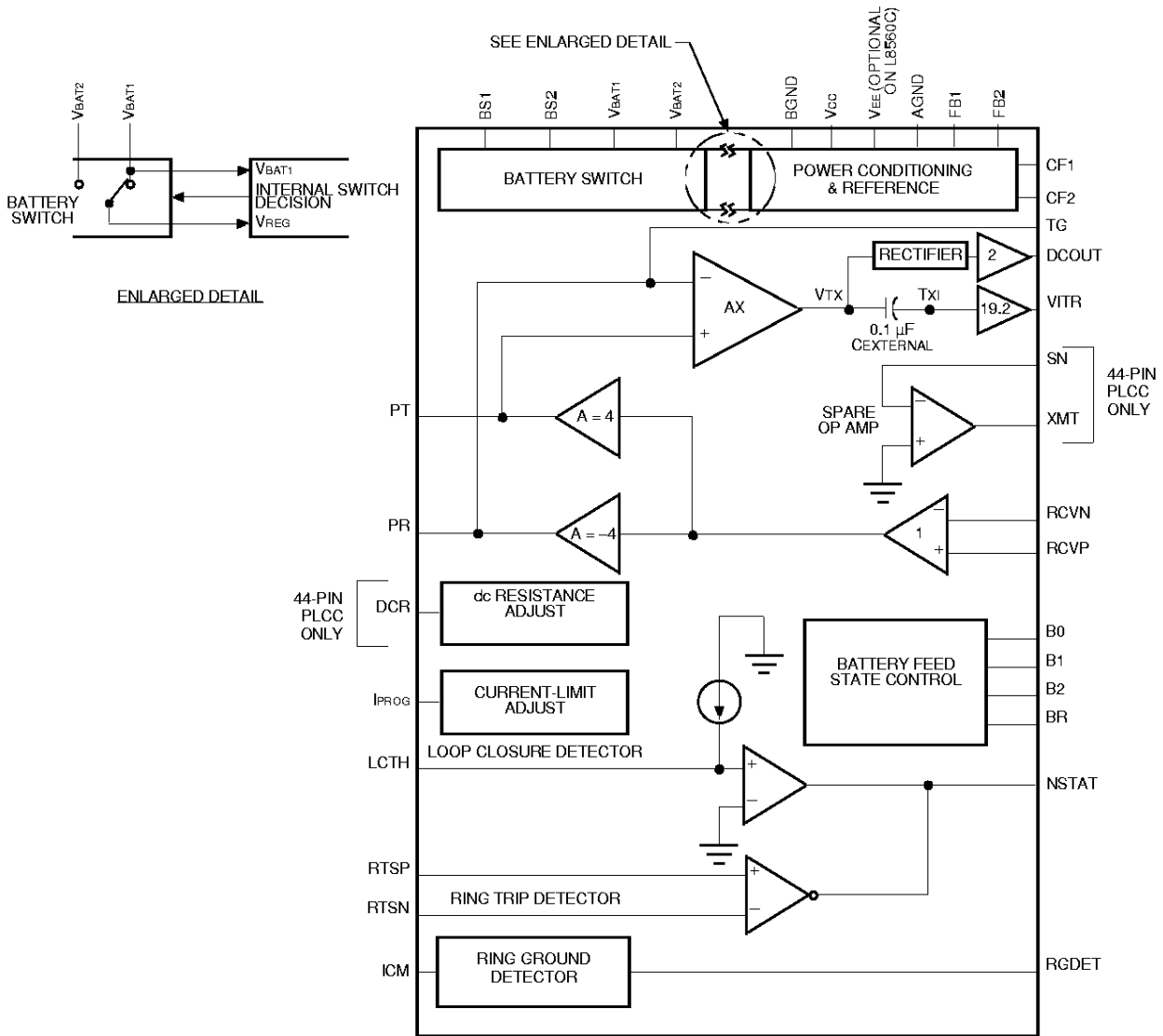
Figure 1. Functional Diagram
