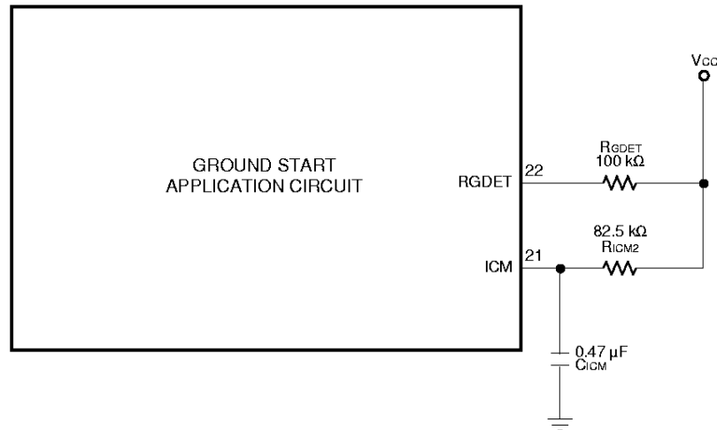
Figure 36. Ground Start Application Circuit
