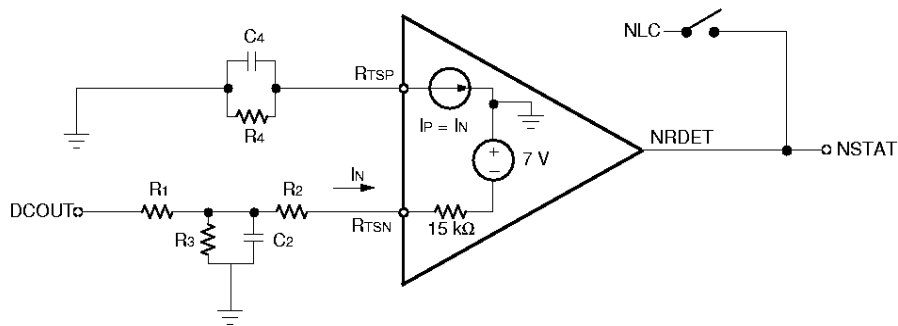
Figure 31. Equivalent Ring Trip Circuit for Balanced Ringing SLIC
