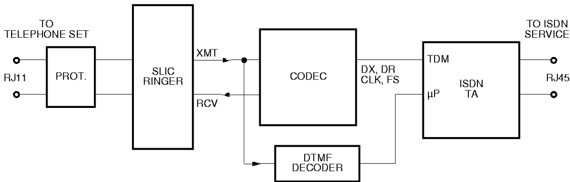
Figure 28. POTS Controlled from an ISDN Terminal Adapter
