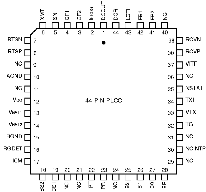
Figure 3. 44-Pin Diagram (PLCC Chip)
