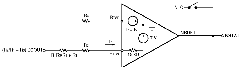
Figure 32. Thevenin Equivalent Ring Trip Circuit for Balanced Ringing SLIC
