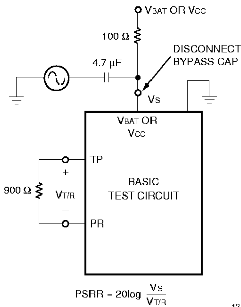
Figure 6. Metallic PSRR
