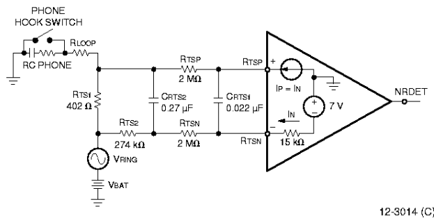
Figure 34. Ring Trip Equivalent Circuit and Equivalent Application
