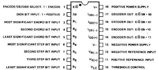
Top View Pin 1 is marked for orientation.
