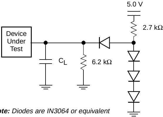
Figure 8. Test Setup
