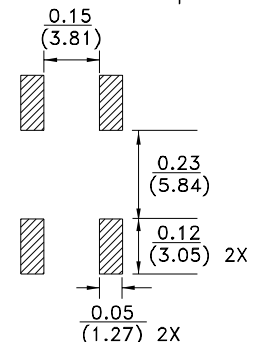
Dimensions: Inches (mm)
