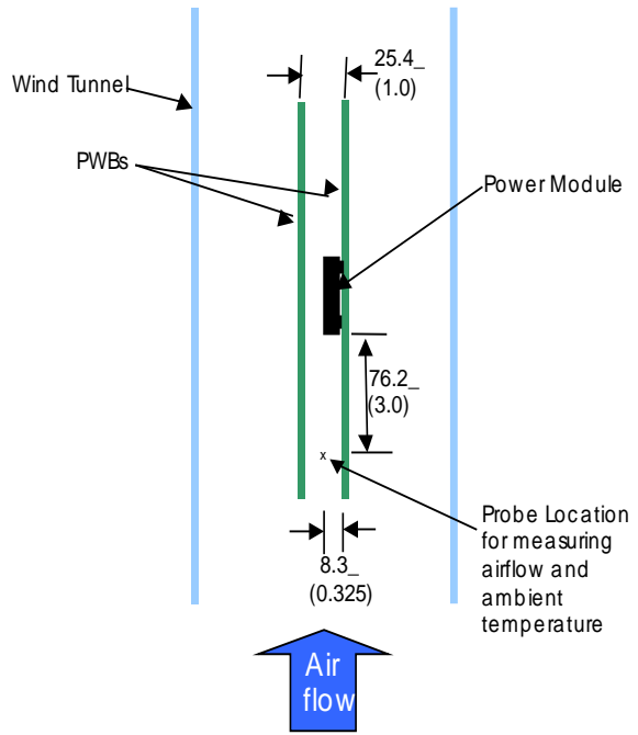
Figure 35. Thermal Test Set-up.
