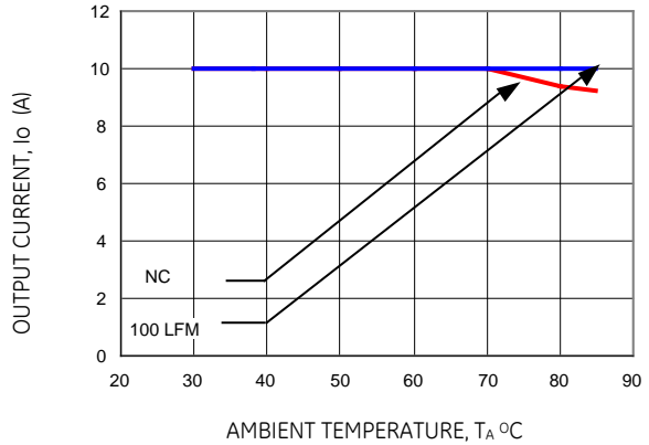
Figure 22. Derating Output Current versus Local Ambient Temperature and Airflow ( V_{in} = 5.0dc , V_o=3.3 Vdc ).
