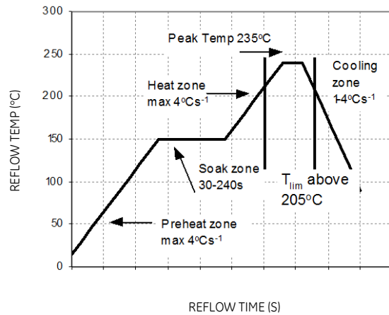
Figure 36. Reflow Profile for Tin/Lead (Sn/Pb) process.
