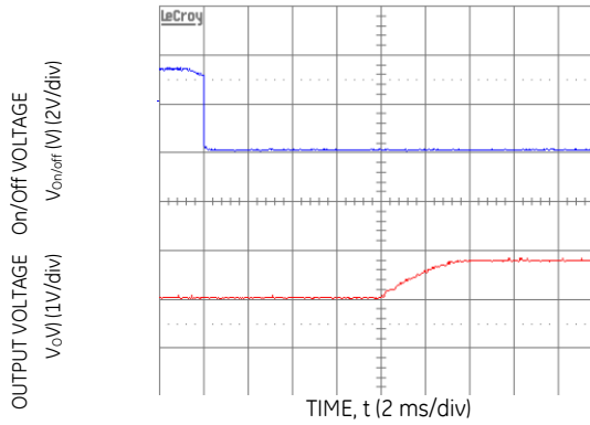
Figure 17. Typical Start-Up with Prebias ( V_{in} = 3.3\text{Vdc} , V_o = 1.8\text{Vdc} , I_o = 1\text{A} , V_{bias} = 1.0\text{Vdc} ).
