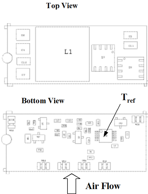
Figure 34. T ref Temperature measurement location.
