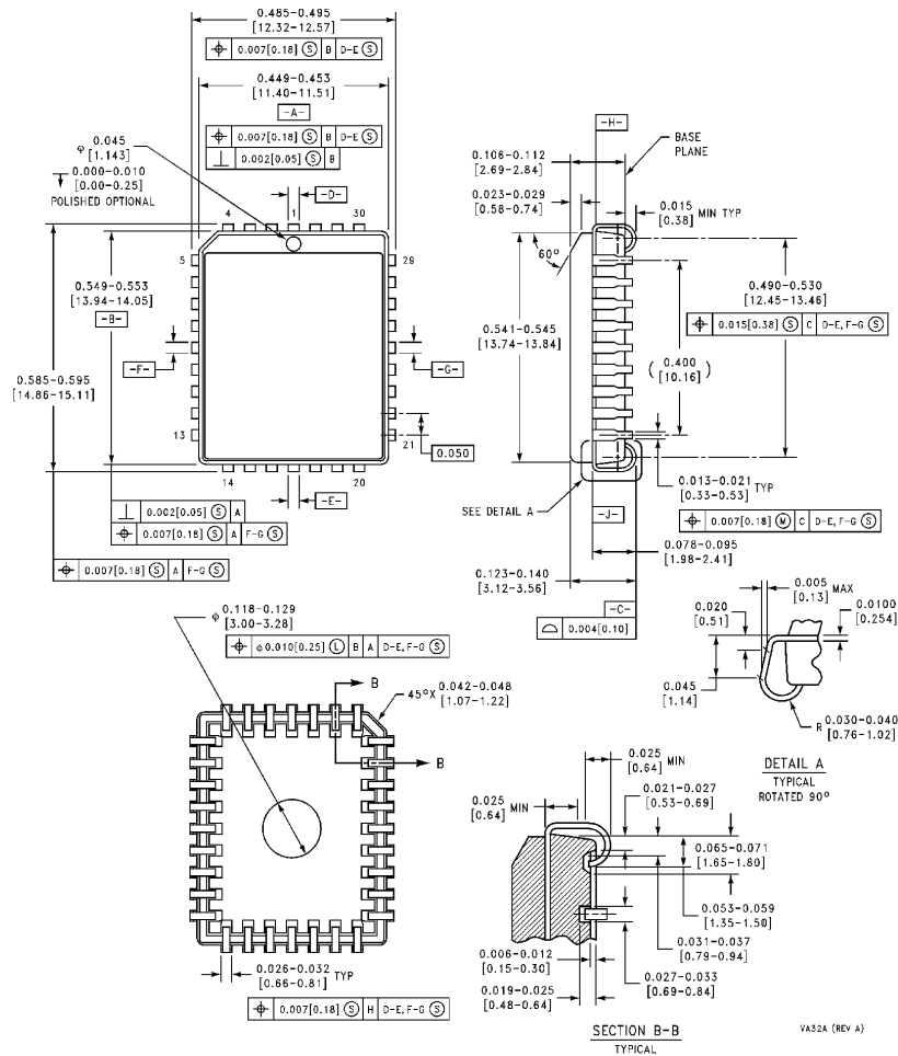
32-Lead Plastic Leaded Chip Carrier (PLCC) Order Number NM27C256VXXX Package Number VA32A
