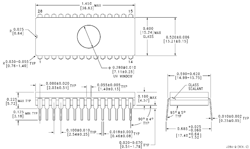
UV Window Cavity Dual-In-Line CerDIP Package (Q) Order Number NM27C256QXXX Package Number J28AQ
